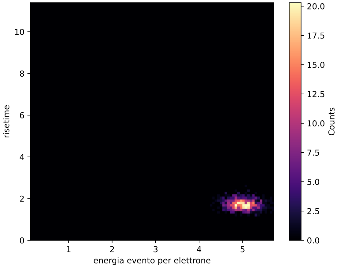
electron distribution 5.0GeV
