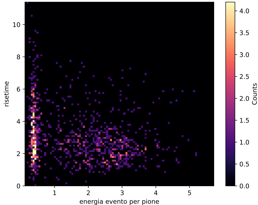
pion distribution 5.0GeV
